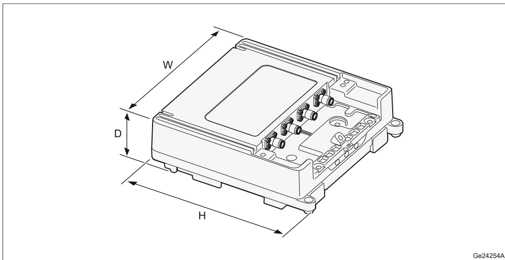
Figure 2 Radio 4402 Dimensions
