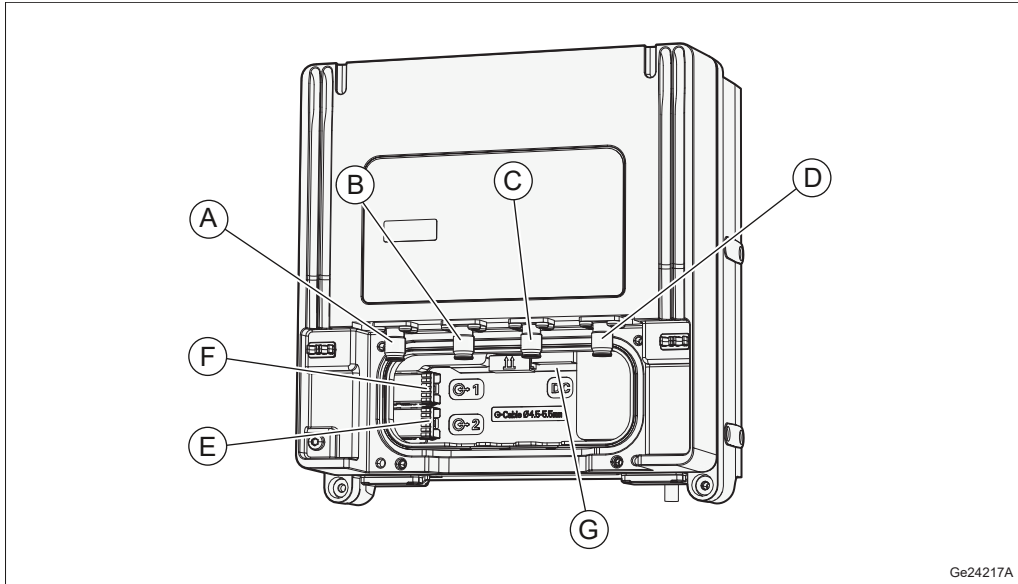
Figure 6 Radio 4402 Connection Interfaces
